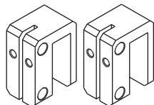
2x LR/LF BRACKETS 16mm (0.6in)
